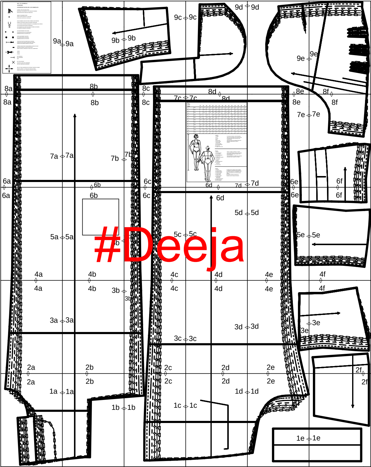
layout drawing
